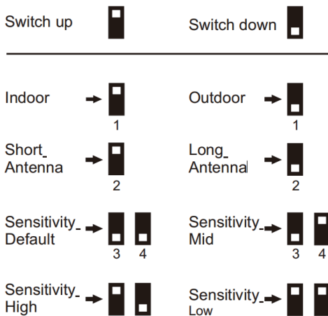
Figure 4 Dip Switch diagram
