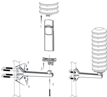
Figure 8 Sensor Mounting
