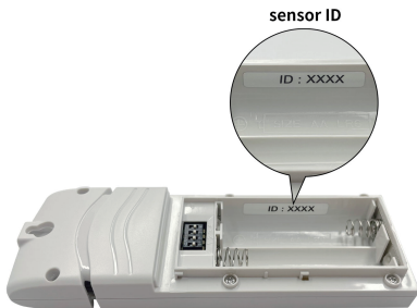
Figure 5 Lightning Sensor
